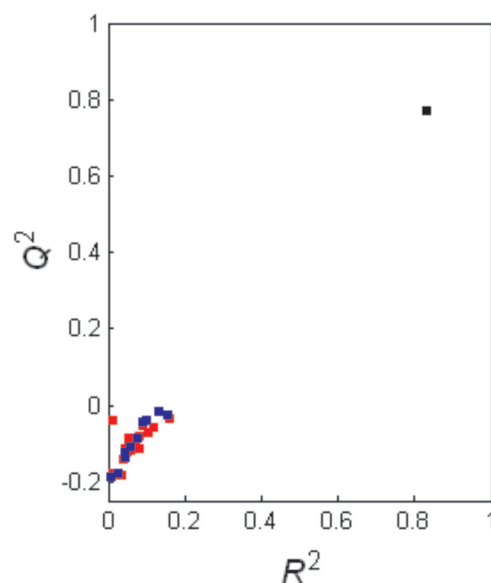
Figure 3. The \mathbf{y} -randomization plot for the MLR model on data set 1: black ball - the real model, blue balls - 10 randomized models, red balls - 25 randomized models.
